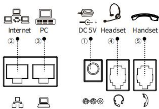
Picture 3 - Connecting to the Device
