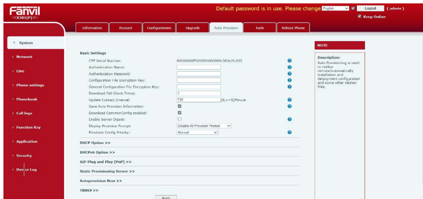
Picture 113 - Page auto provision Settings
