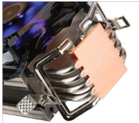
Four high performance heatpipes and 8mm thick copper coldplate work together to quickly transfer heat away from your CPU
