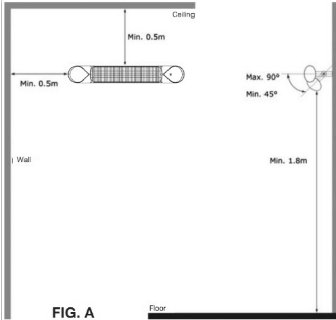
Diagram 2: Correct Wall / Ceiling Position
