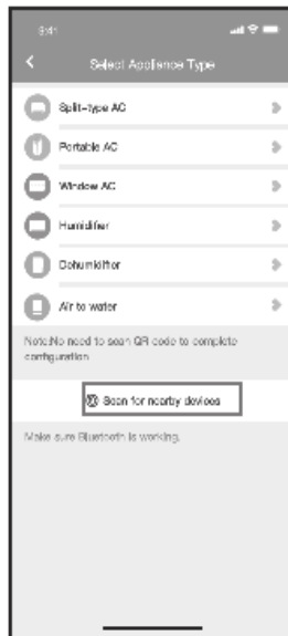
iOS
