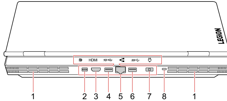
Figure 5. Lenovo Legion Y740–15/17 Series – rear view
