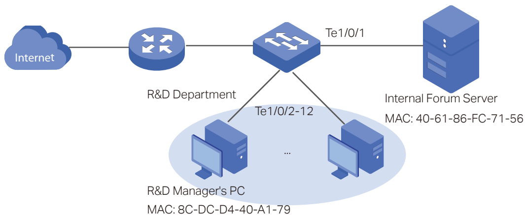
Figure 3-1 Network Topology
