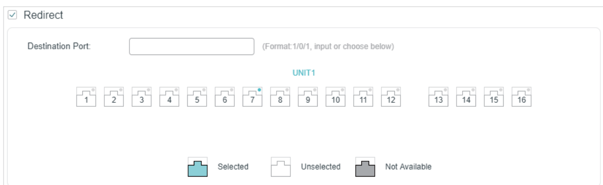
Figure 2-18 Configuring Redirect
