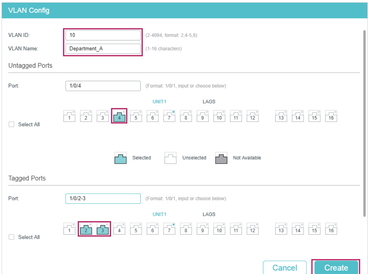
Figure 3-6 Creating VLAN 10
