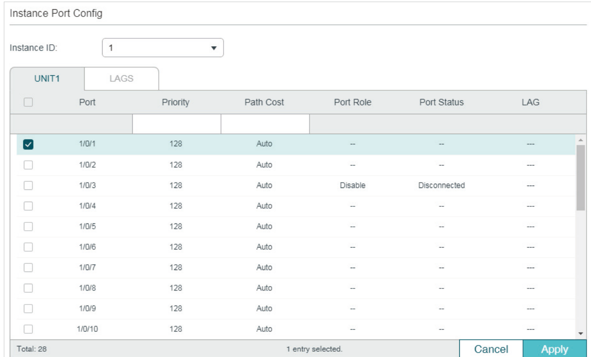
Figure 3-5 Configuring Port Parameters in the Instance
