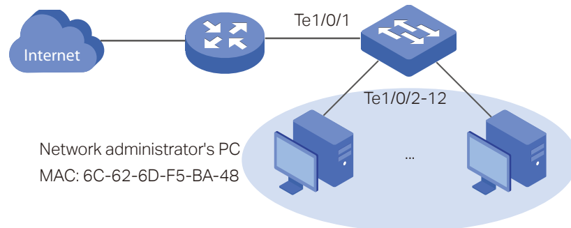
Figure 3-23 Network Topology
