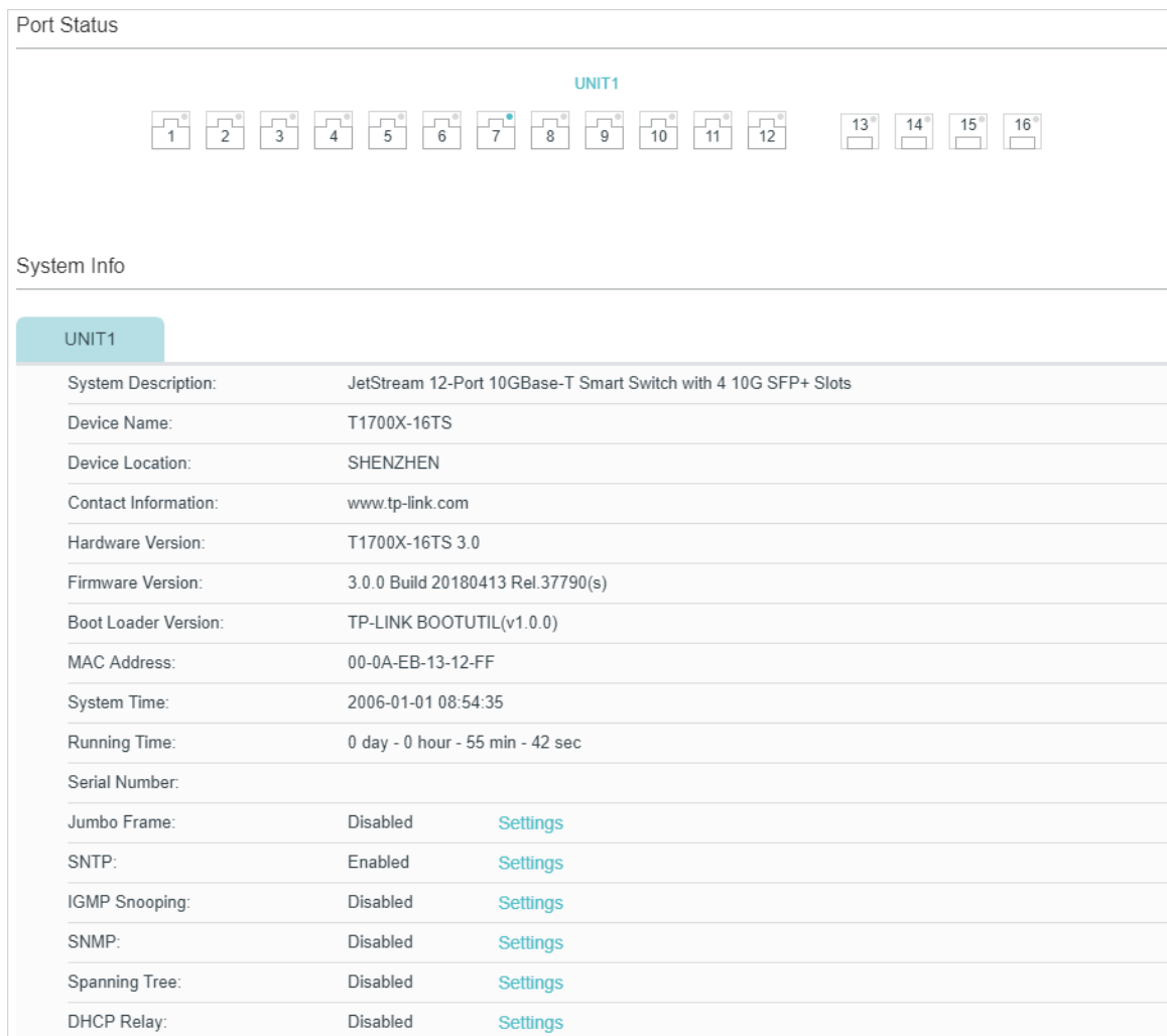
Figure 2-3 Web interface
