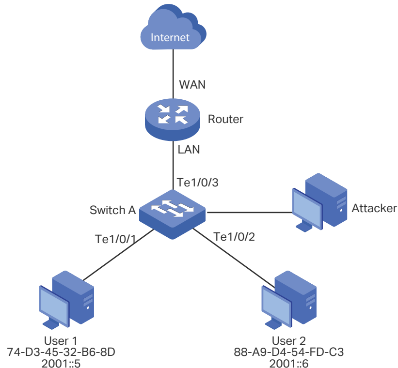
Figure 5-1 Network Topology
