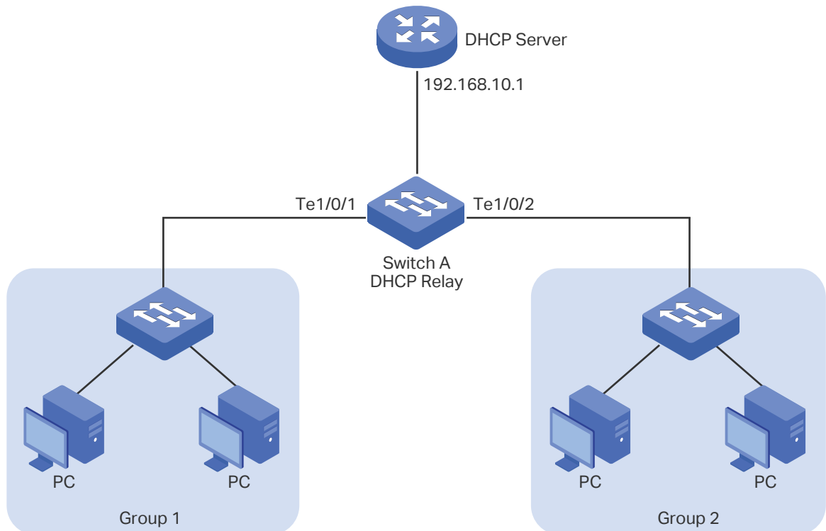
Figure 5-1 Network Topology for DHCP L2 Relay
