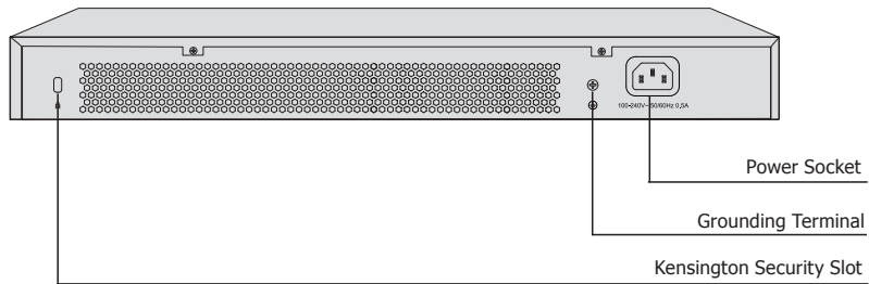
Figure 1-3 Rear Panel
